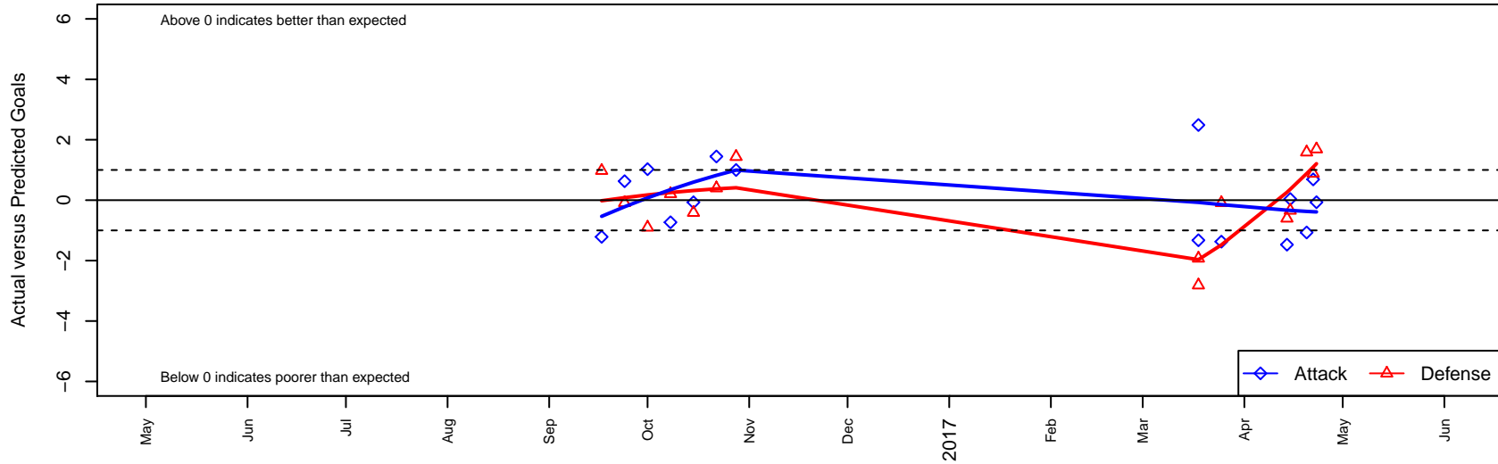
SSC Shadow Elite B06 Dots are actual minus expected GF (blue circles) and GA (red triangles). Blue line is smoothed change in attack strength. Red is smoothed change in defense strength.
